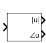
Fourier
